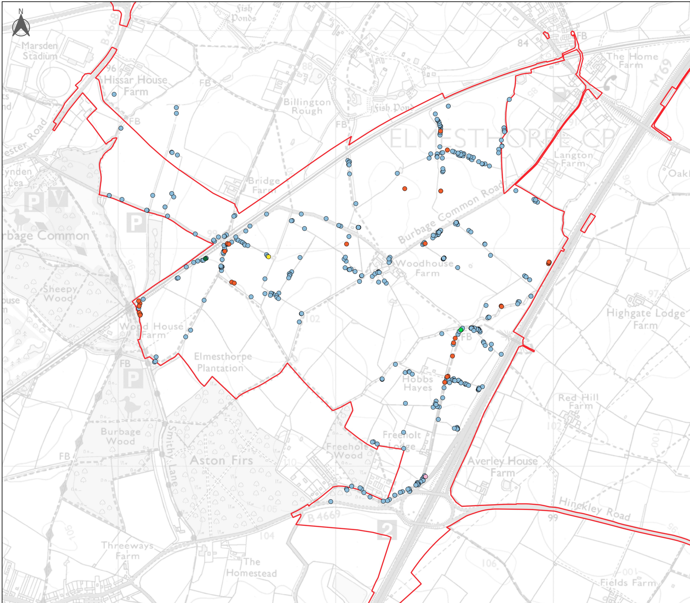
Figure 12.17: Bat Transect Survey Results – July 2021 (Dusk)
